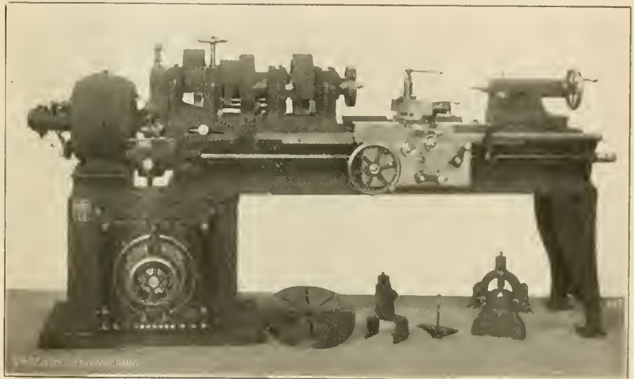
LODGE & SHIPLEY PATENT HEAD MOTOR DRIVEN LATHE.
